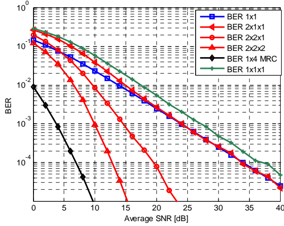
Fig. 2. BER for dual-hop dual-antenna MAF systems.
