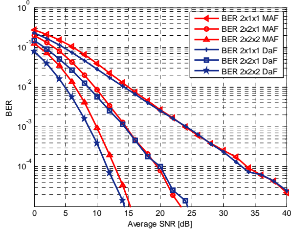
Fig. 3. BER for dual-hop and dual-antenna MAF and DF systems.
